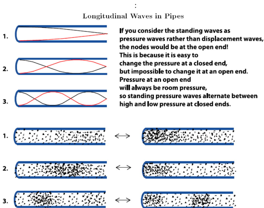
Figure 3.10 Longitudinal Wave in Pipes The standing waves in the tubes are actually longitudinal sound waves. Here the displacement standing waves in Figure 3.10 are shown instead as longitudinal air pressure waves. Each wave would be oscillating back and forth between the state on the right and the one on the left.
