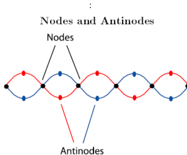
Figure 3.7 Nodes and Antinodes As a standing wave waves back and forth (from the red to the blue position), there are some spots called nodes that do not move at all; basically there is no change, no waving up- and-down (or back-and-forth), at these spots. The spots at the biggest part of the wave – where there is the most change during each wave – are called antinodes.
