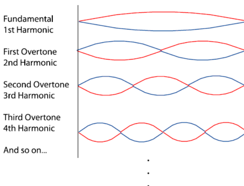
Figure 3.6 Standing Wave Harmonics There is a whole set of standing waves, called harmonics, that will fit into any "container" of a specific length. This set of waves is called a harmonic series.
