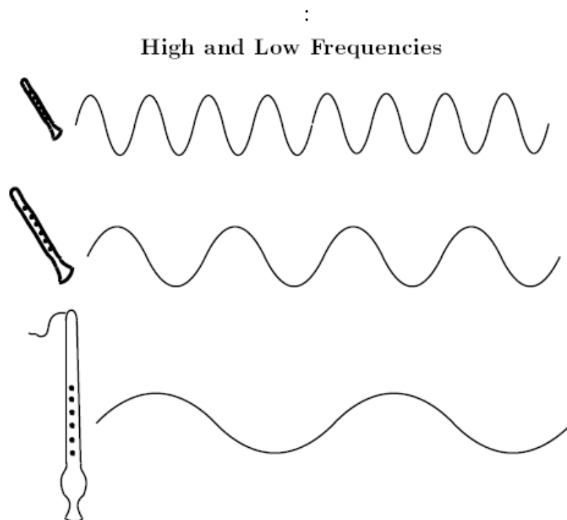
Figure 4.1 High and Low Frequencies A sound that has a shorter wavelength has a higher frequency and a higher pitch.
