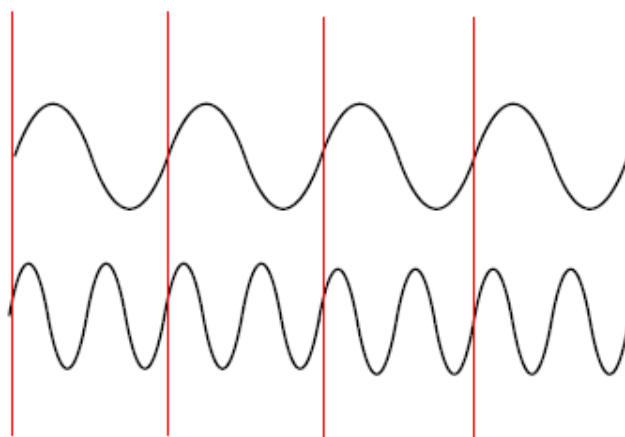
Figure 4.2 Octave Frequencies When two notes are one octave apart, one has a frequency exactly two times higher than the other - it has twice as many waves. These waves fit together so well, in the instrument, and in the air, and in your ears, that they sound almost like different versions of the same note.
