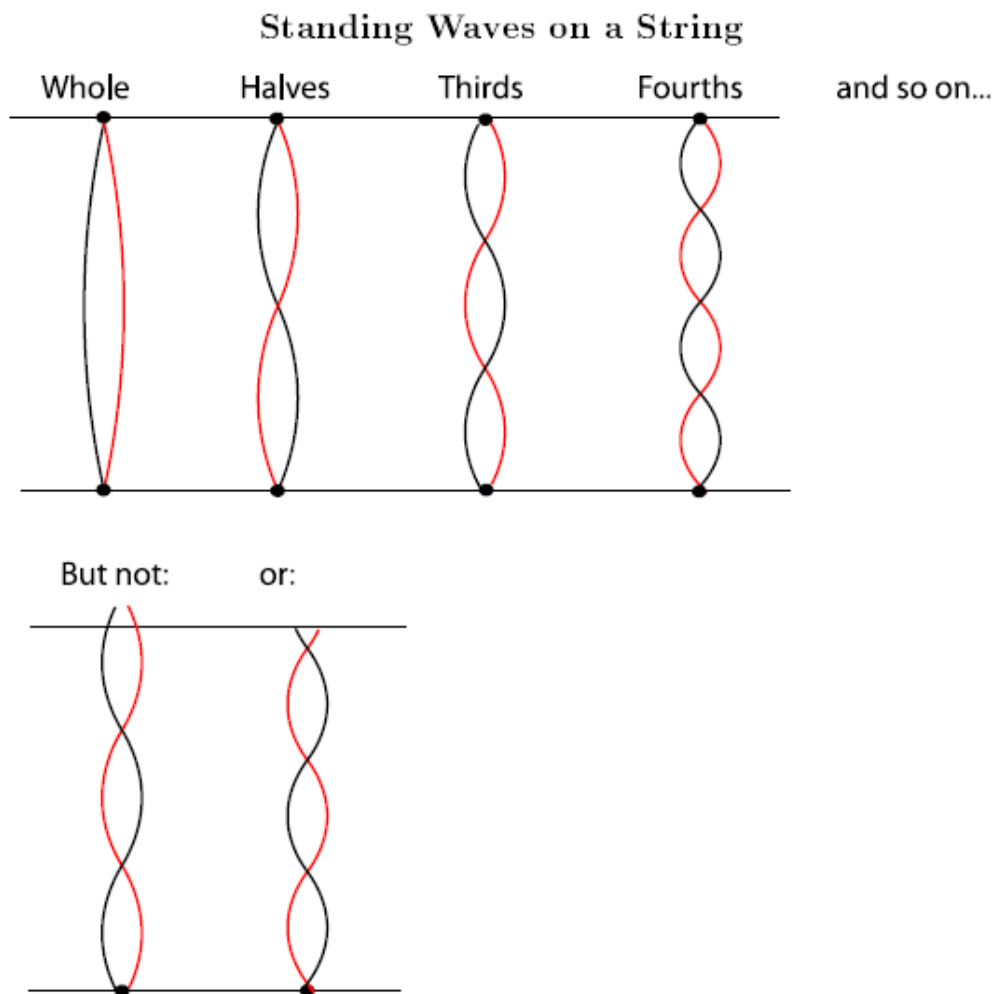
Figure 3.8 Standing Waves on a String A string that's held very tightly at both ends can only vibrate at very particular wavelengths. The whole string can vibrate back and forth. It can vibrate in halves, with a node at the middle of the string as well as each end, or in thirds, fourths, and so on. But any wavelength that doesn't have a node at each end of the string, can't make a standing wave on the string. To get any of those other wavelengths, you need to change the length of the vibrating string. That is what happens when the player holds the string down with a finger, changing the vibrating length of the string and changing where the nodes are.
