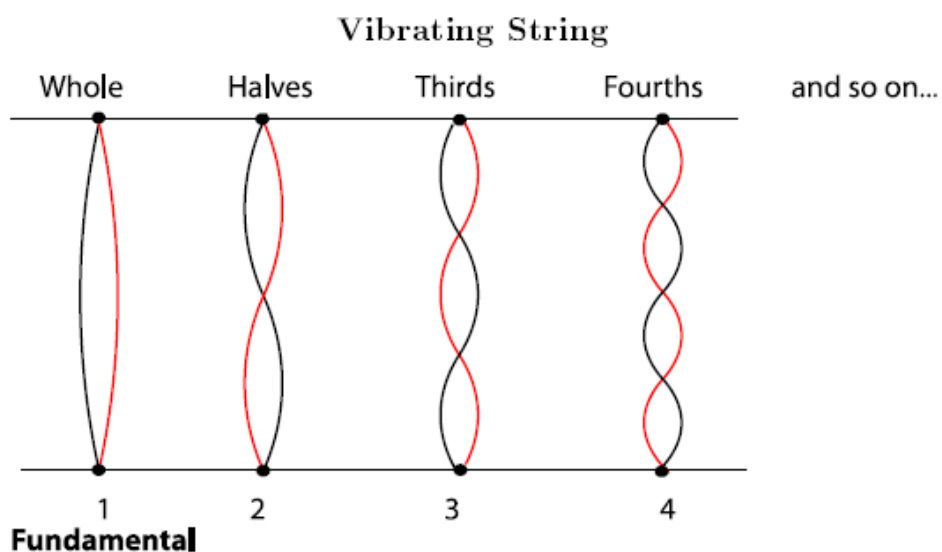
Figure 3.12 Vibrating String The fundamental pitch is produced by the whole string vibrating back and forth. But the string is also vibrating in halves, thirds, quarters, fifths, and so on, producing harmonics. All of these vibrations happen at the same time, producing a rich, complex, interesting sound.
