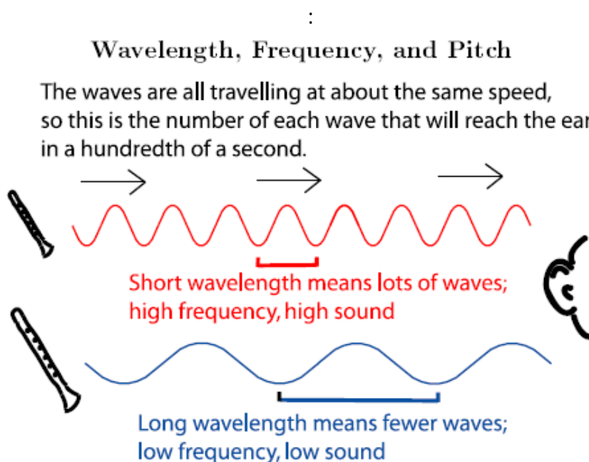
Figure 3.4 Wavelength, Frequency, and Pitch Since the sounds are travelling at about the same speed, the one with the shorter wavelength "waves" more frequently; it has a higher frequency, or pitch. In other words, it sounds higher.
