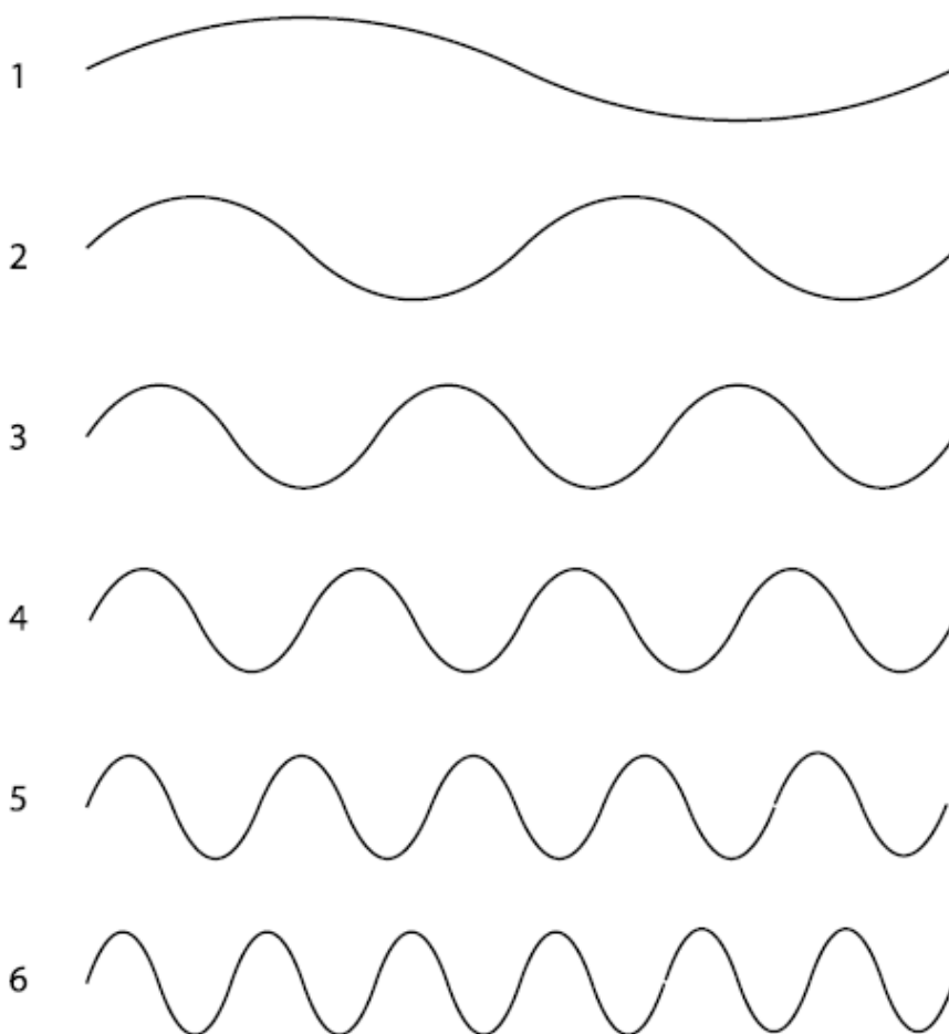
Figure 3.13 Harmonic Series Wavelengths and Frequencies The second harmonic has half the wavelength and twice the frequency of the first. The third harmonic has a third the wavelength and three times the frequency of the first. The fourth harmonic has a quarter the wavelength and four times the frequency of the first, and so on. Notice that the fourth harmonic is also twice the frequency of the second harmonic, and the sixth harmonic is also twice the frequency of the third harmonic.
