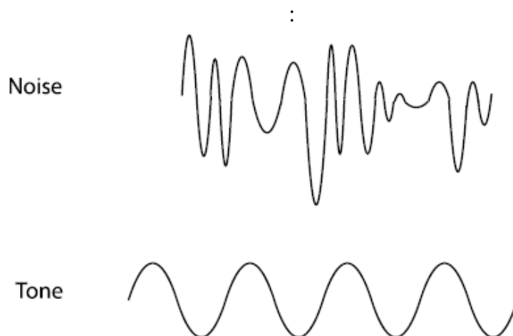
Figure 3.1 A random jumble of sound waves is heard as a noise. A regular, evenly-spaced sound wave is heard as a tone.
