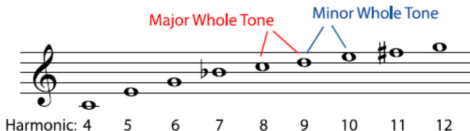
Figure 6.3 Just intonation Both the 9:8 ratio and the 10:9 ratio in the harmonic series are written as whole notes. 9:8 is considered a major whole tone and 10:9 a minor whole tone. The difference between them is less than a quarter of a semitone.
